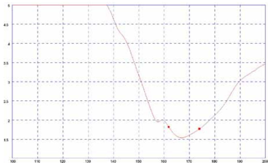
Typical VSWR
