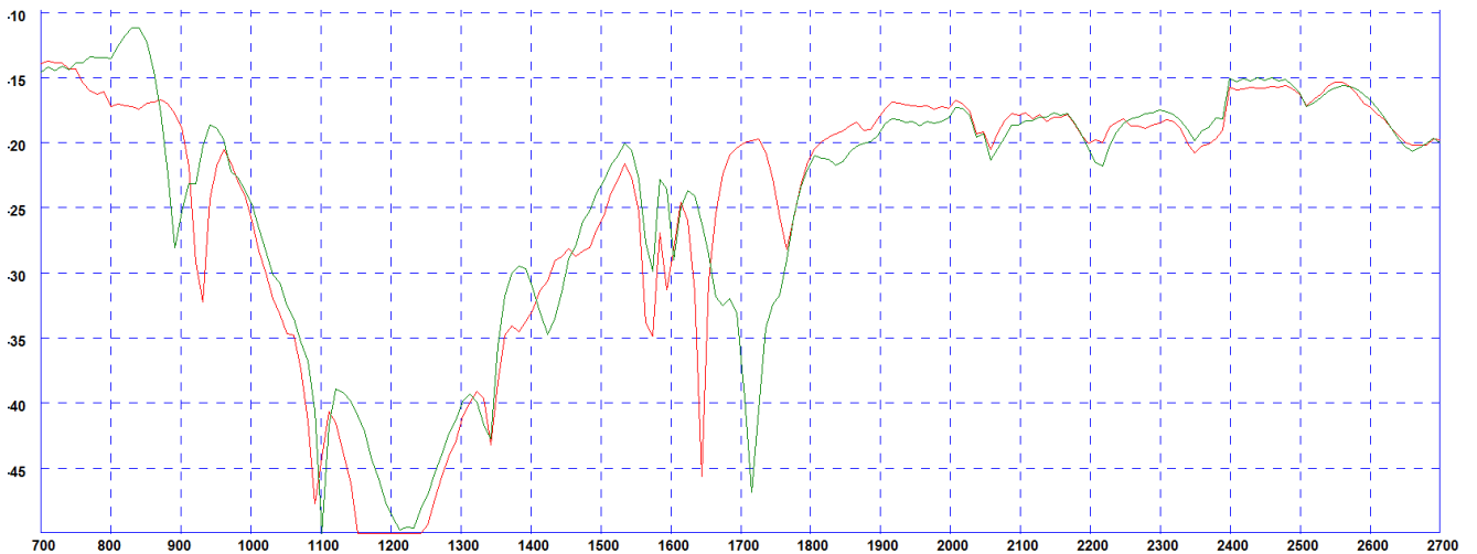
Typical Isolation - WiFi Elements 4&5*
